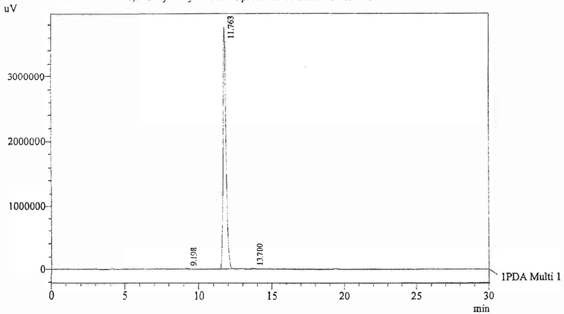
Chromatogram 7,3'-Dihydroxyflavone D:\promonence\Data\2013\APR-2013\020413J.lcd
